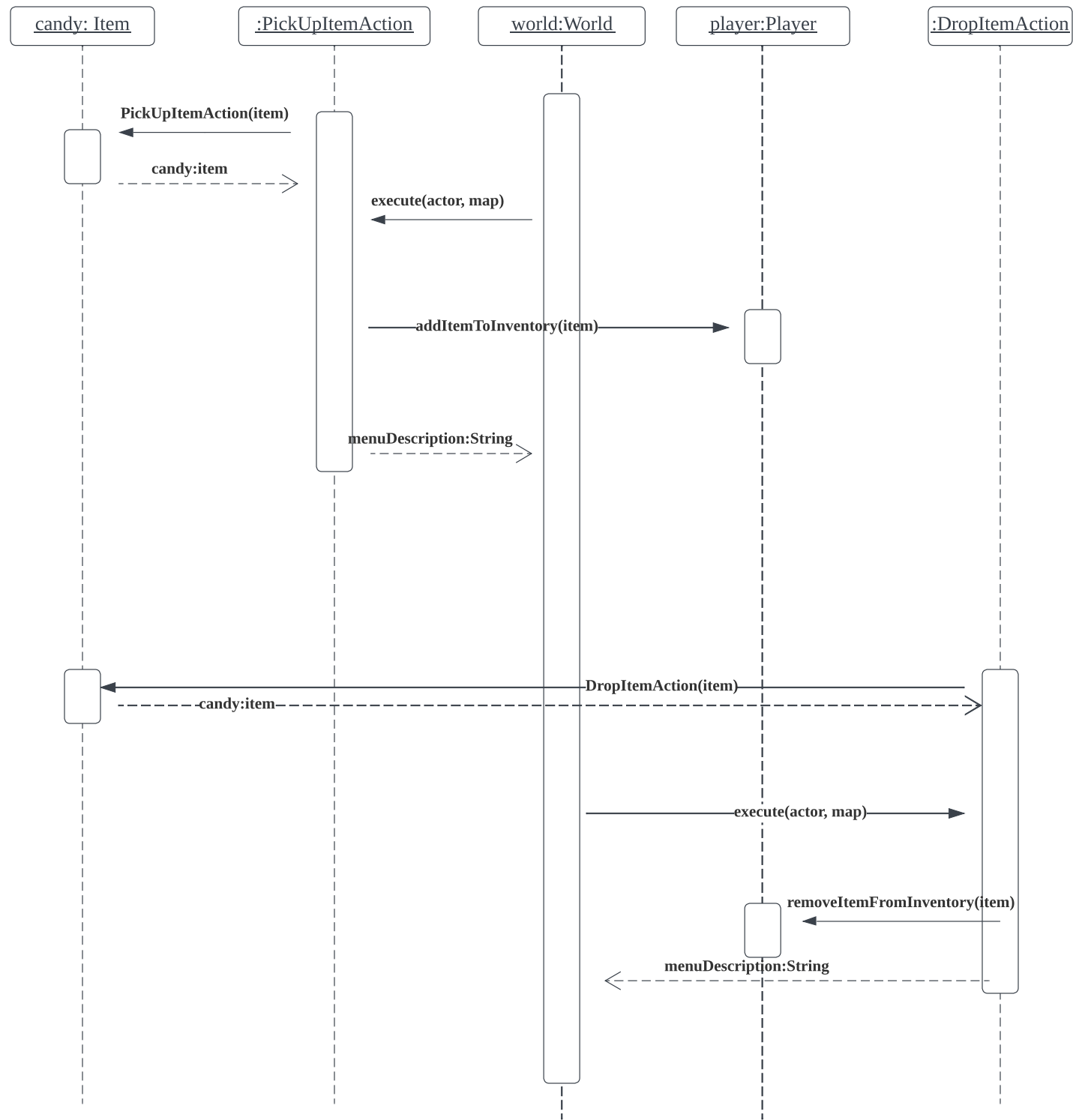
Sequence Diagram: Picking up Candy and Dropping it
